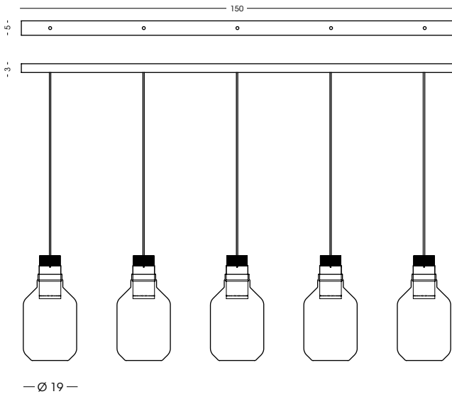
1427.150.5L Binario a soffitto / Ceiling track vetro/glass Ø19 cm - cavo/cable 200 cm 5x LED 10W - 3000 K - 900 lm - 230V CE IP20 1m
