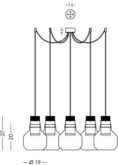
1413.5L Sospensione / Hanging lamp vetro/glass Ø19 cm - cavo/cable 200 cm 5x LED 10W - 3000 K - 900 lm - 230V CE IP20 1m
