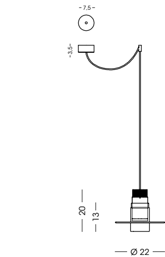
1403.1LD Sospensione / Hanging lamp vetro/glass Ø22 cm - cavo/cable 200 cm 1x LED 10W - 3000 K - 900 lm - 230V CE IP20 1m
