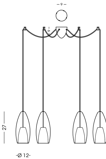
1393.4L Sospensione / Hanging lamp vetro/glass Ø12 cm - cavo/cable 200 cm 4 E14 x 60W 220-240V CE IP20 1m
