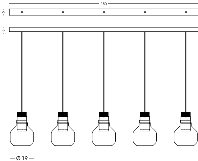
1417.150.5L Binario a soffitto / Ceiling track vetro/glass Ø19 cm - cavo/cable 200 cm 5x LED 10W - 3000 K - 900 lm - 230V CE IP20 1m
