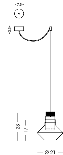
1443.1LD Sospensione / Hanging lamp vetro/glass Ø21 cm - cavo/cable 200 cm 1x LED 10W - 3000 K - 900 lm - 230V CE IP20 1m
