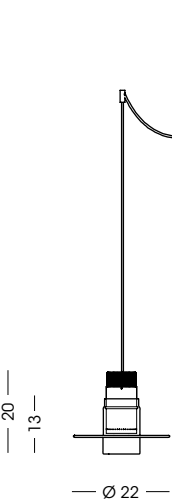
1403.2L Sospensione / Hanging lamp vetro/glass Ø22 cm - cavo/cable 200 cm 2x LED 10W - 3000 K - 900 lm - 230V CE IP20 1m
