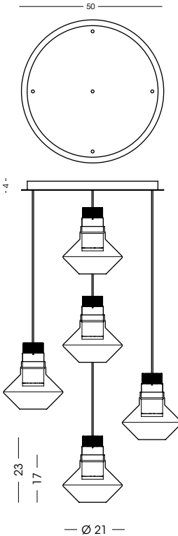
1449.50.5L Plafoniera / Ceiling lamp vetro/glass Ø21 cm - cavo/cable 200 cm 5x LED 10W - 3000 K - 900 lm - 230V CE IP20 1m
