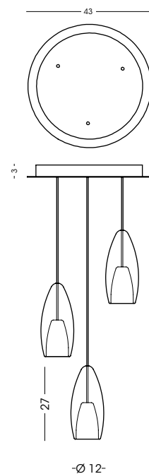
1397.120.3L Binario a soffitto / Ceiling track vetro/glass Ø12 cm - cavo/cable 200 cm 3 E14 x 60W 220-240V CE IP20 1m
