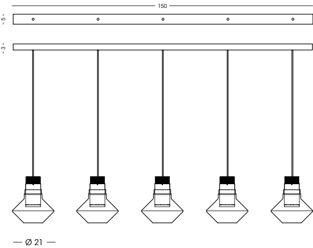
1447.150.5L Binario a soffitto / Ceiling track vetro/glass Ø21 cm - cavo/cable 200 cm 5x LED 10W - 3000 K - 900 lm - 230V CE IP20 1m
