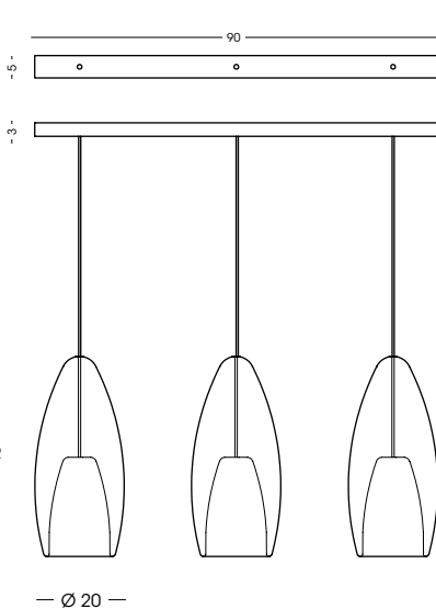
XXL1397.90.3L Binario a soffitto / Ceiling track vetro/glass Ø20 cm - cavo/cable 200 cm 💡 3 E27 x 105W 220-240V CE IP20 1m
