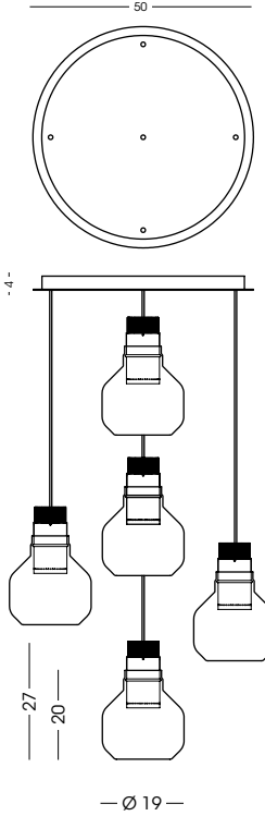
1419.50.5L Plafoniera / Ceiling lamp vetro/glass Ø19 cm - cavo/cable 200 cm 5x LED 10W - 3000 K - 900 lm - 230V CE IP20 1m
