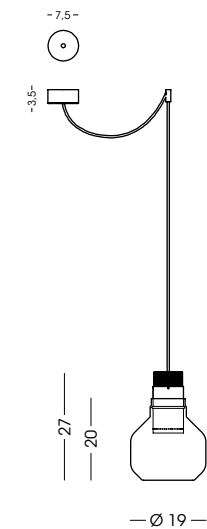
1413.1LD Sospensione / Hanging lamp vetro/glass Ø19 cm - cavo/cable 200 cm 1x LED 10W - 3000 K - 900 lm - 230V CE IP20 1m
