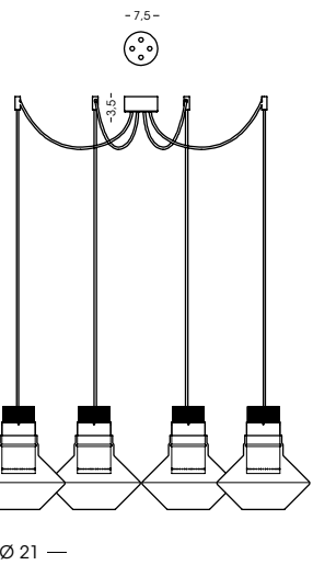
1443.4L Sospensione / Hanging lamp vetro/glass Ø21 cm - cavo/cable 200 cm 4x LED 10W - 3000 K - 900 lm - 230V CE IP20 1m
