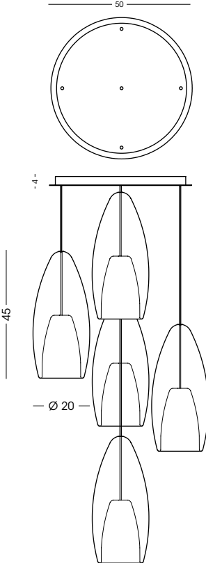
XXL1399.50.5L Plafoniera / Ceiling lamp vetro/glass Ø20 cm - cavo/cable 200 cm 💡 5 E27 x 105W 220-240V CE IP20 1m
