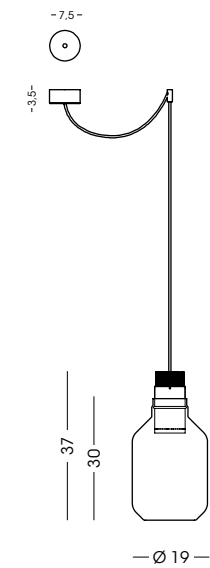
1423.1LD Sospensione / Hanging lamp vetro/glass Ø19 cm - cavo/cable 200 cm 1x LED 10W - 3000 K - 900 lm - 230V CE IP20 1m
