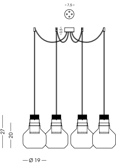
1413.4L Sospensione / Hanging lamp vetro/glass Ø19 cm - cavo/cable 200 cm 4x LED 10W - 3000 K - 900 lm - 230V CE IP20 1m
