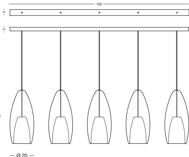
XXL1397.150.5L Binario a soffitto / Ceiling track vetro/glass Ø20 cm - cavo/cable 200 cm 💡 5 E27 x 105W 220-240V CE IP20 1m
