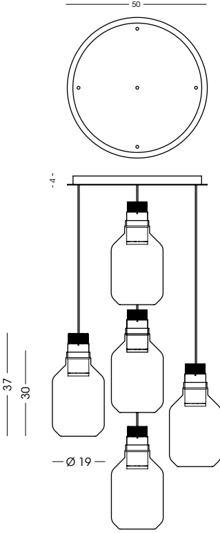
1429.50.5L Plafoniera / Ceiling lamp vetro/glass Ø19 cm - cavo/cable 200 cm 5x LED 10W - 3000 K - 900 lm - 230V CE IP20 1m
