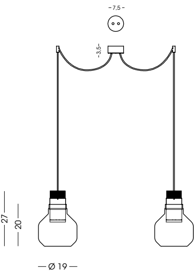
1413.2L Sospensione / Hanging lamp vetro/glass Ø19 cm - cavo/cable 200 cm 2x LED 10W - 3000 K - 900 lm - 230V CE IP20 1m
