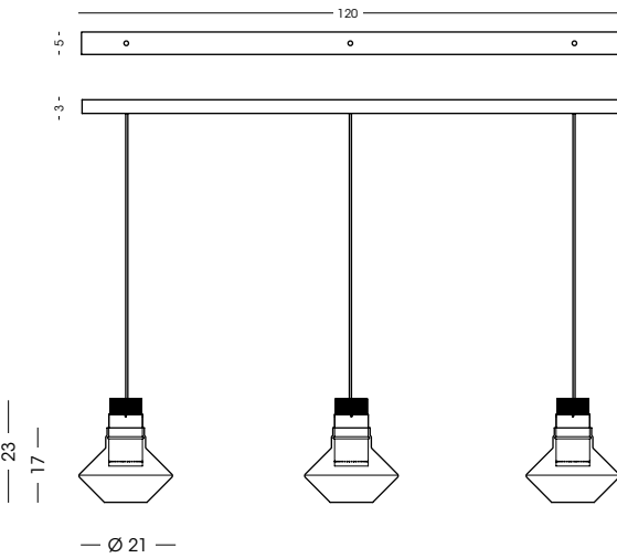
1447.120.3L Binario a soffitto / Ceiling track vetro/glass Ø21 cm - cavo/cable 200 cm 3x LED 10W - 3000 K - 900 lm - 230V CE IP20 1m
