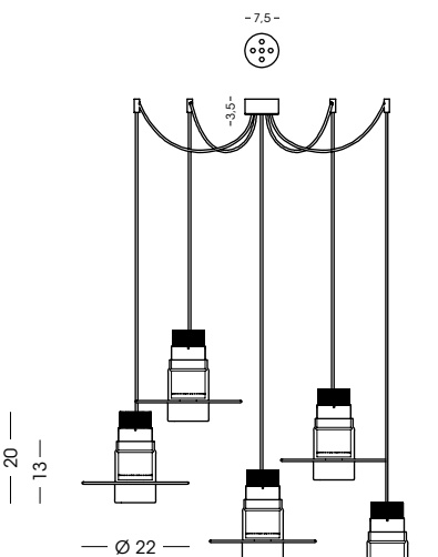
1403.5L Sospensione / Hanging lamp vetro/glass Ø22 cm - cavo/cable 200 cm 5x LED 10W - 3000 K - 900 lm - 230V CE IP20 1m
