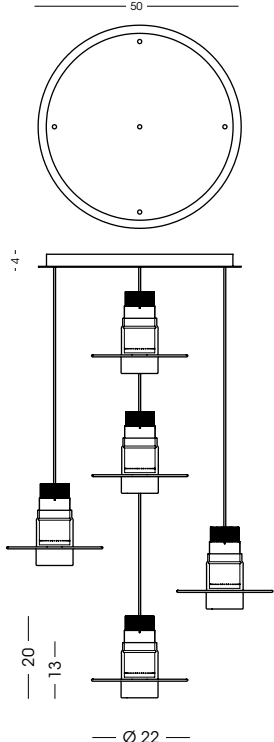
1409.50.5L Plafoniera / Ceiling lamp vetro/glass Ø22 cm - cavo/cable 200 cm 5x LED 10W - 3000 K - 900 lm - 230V CE IP20 1m
