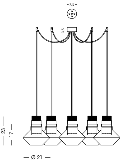
1443.5L Sospensione / Hanging lamp vetro/glass Ø21 cm - cavo/cable 200 cm 5x LED 10W - 3000 K - 900 lm - 230V CE IP20 1m
