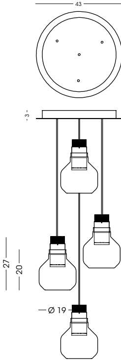
1419.43.4L Plafoniera / Ceiling lamp vetro/glass Ø19 cm - cavo/cable 200 cm 4x LED 10W - 3000 K - 900 lm - 230V CE IP20 1m
