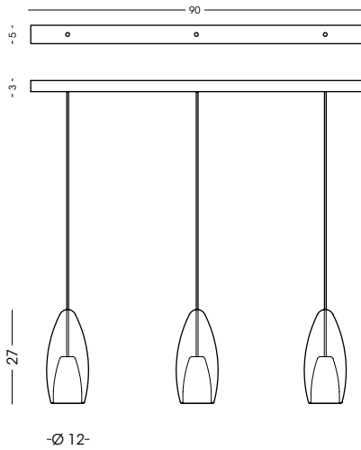
1397.90.3L Binario a soffitto / Ceiling track vetro/glass Ø12 cm - cavo/cable 200 cm 3 E14 x 60W 220-240V CE IP20 1m
