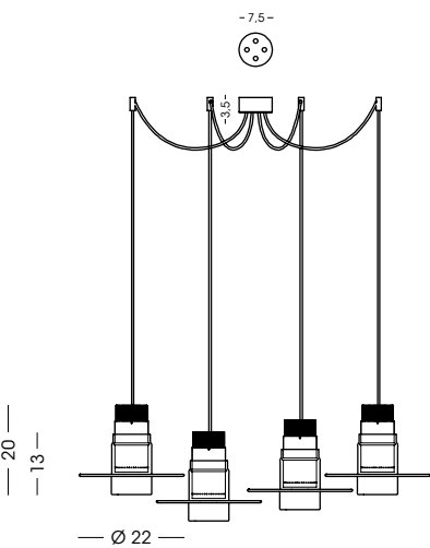
1403.4L Sospensione / Hanging lamp vetro/glass Ø22 cm - cavo/cable 200 cm 4x LED 10W - 3000 K - 900 lm - 230V CE IP20 1m
