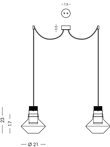
1443.2L Sospensione / Hanging lamp vetro/glass Ø21 cm - cavo/cable 200 cm 2x LED 10W - 3000 K - 900 lm - 230V CE IP20 1m
